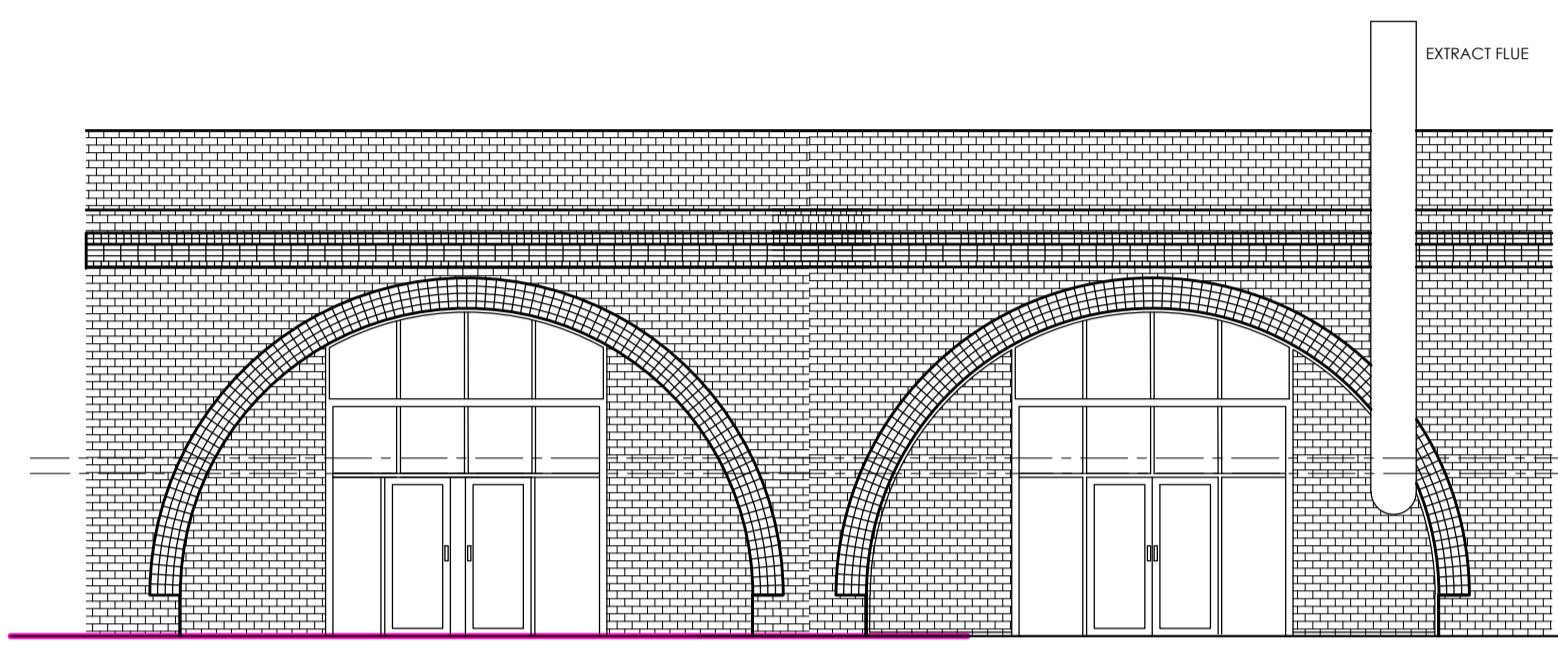
PROPOSED FRONT ELEVATION (ARCH 148)
